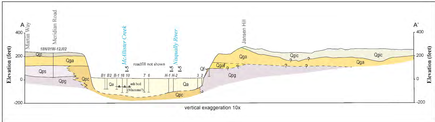
6 7 Figure D-36. Cross-Section of Study Area along I-5 (Walsh et al., 2003)
