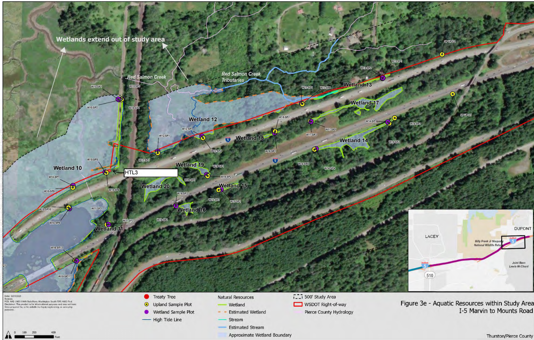
Figure D-13. Wetland Boundaries and Stream Locations (e)
